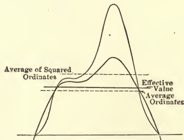
FIG. 42. Current wave and square of same, showing derivation of "effective" value of an alternating quantity.
